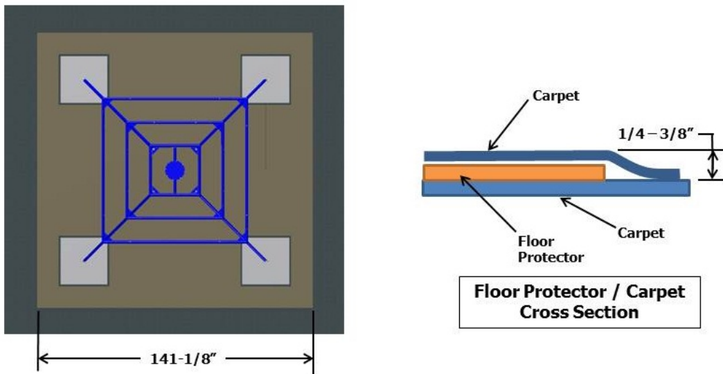
Figure 2-8: PYRAMID Floor Protectors
